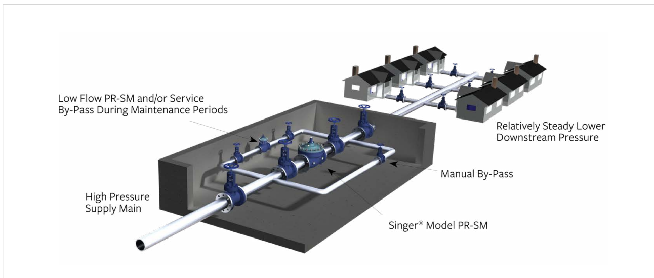
FIG. 1 Typical application
