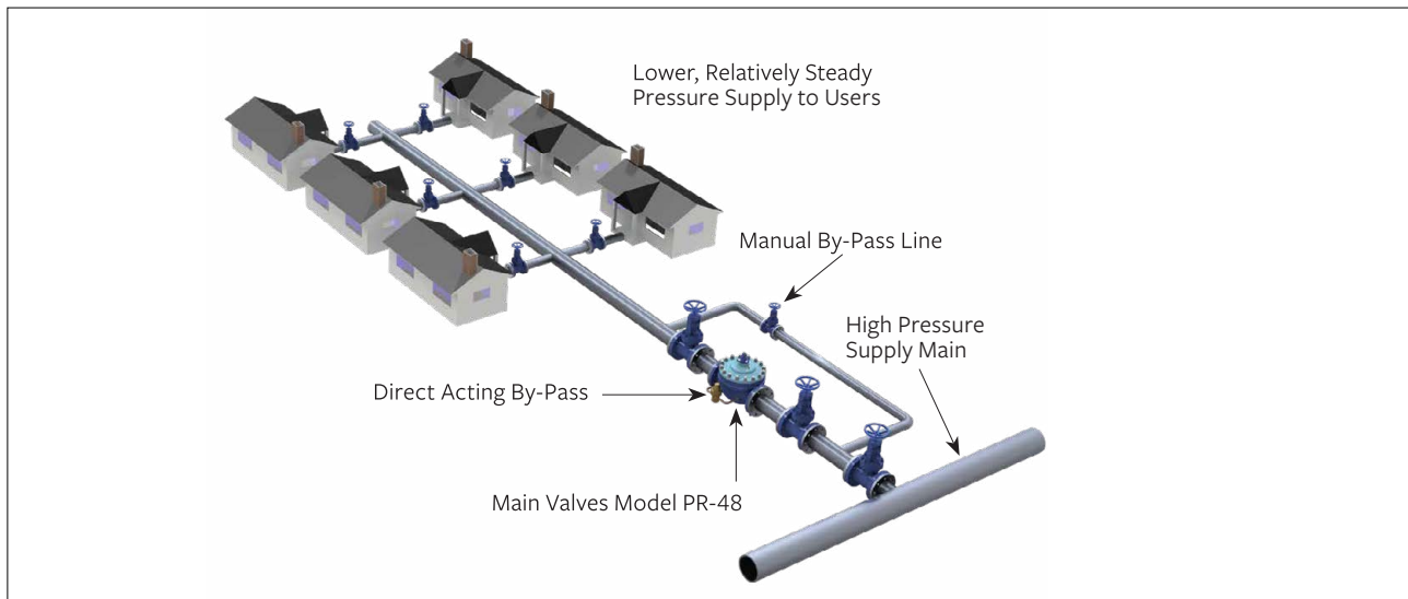
FIG. 1 Typical application
