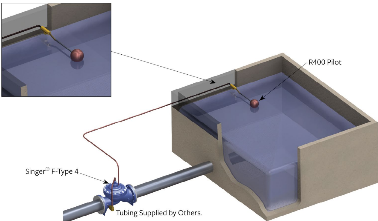
FIG. 1 Typical application
