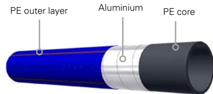
FIG. 1 Puriton Pipe Structure
