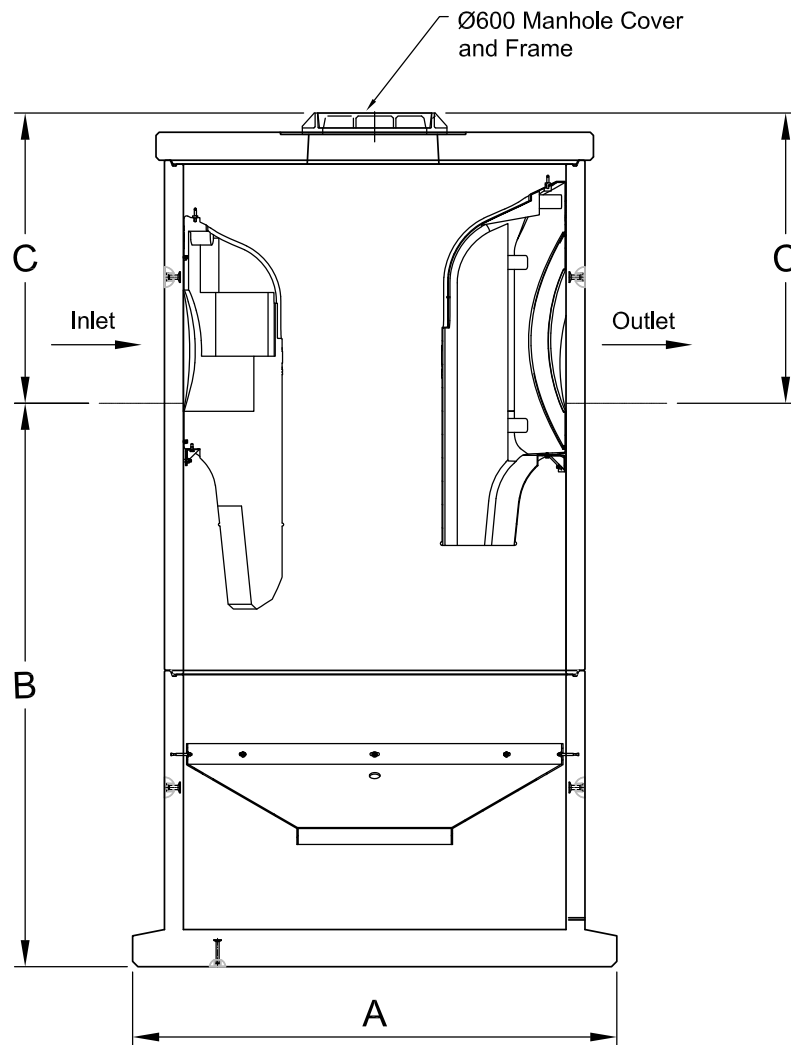
FIG. 1 Downstream Defender® Select concrete chamber dimension drawing
