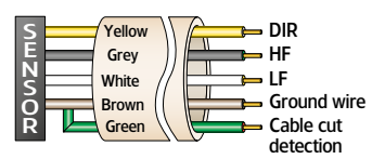
» 5-wires
