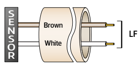
» 2-wires
