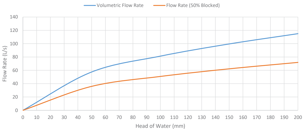
Flow Rate Estimate TP800DG
