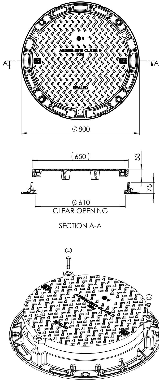
FIG. 1 TP800 Bolt Down Cover Drawing
