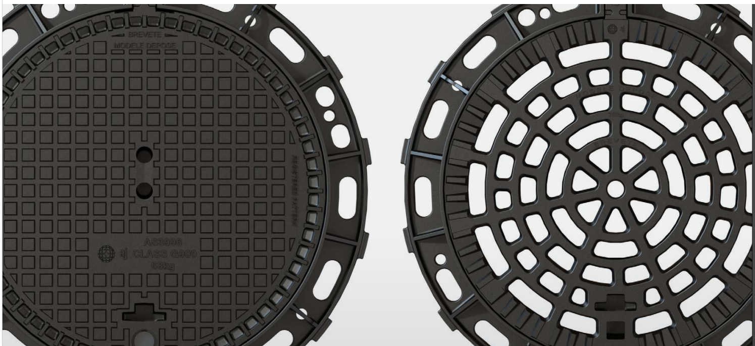
02.21 | DRAINAGE | D16.11 EJ SOLO 600MM F900 HINGED COVERS AND GRATES
